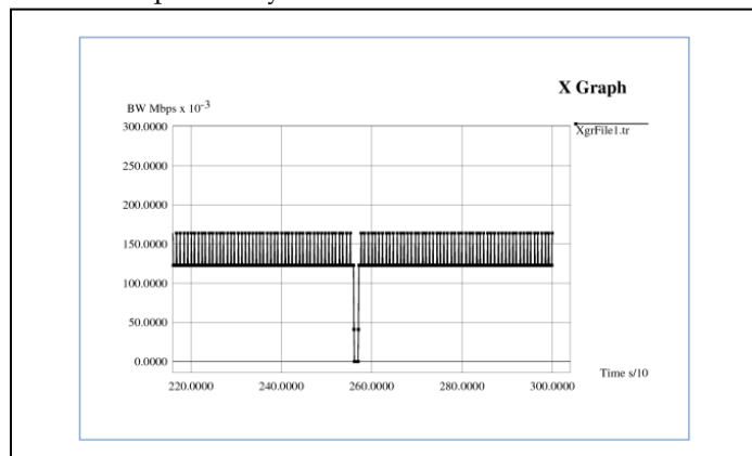
Fig. 16. Link Usage for Seamless MIP.
