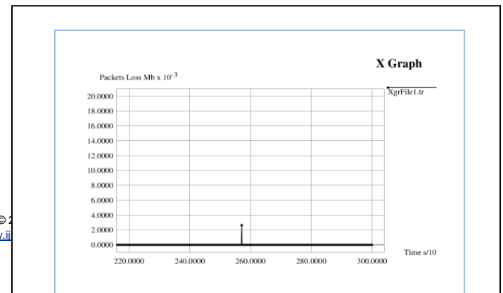
Fig. 18. Packet Loss for Seamless MIP.
